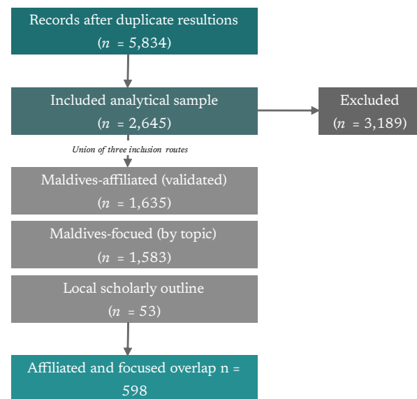
Figure 1. Dataset construction, validation, and final analytical sample
